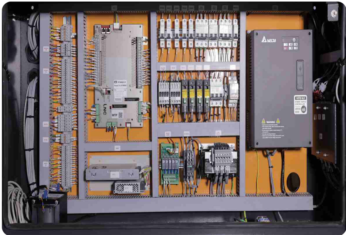
ELECTRICAL PANEL
